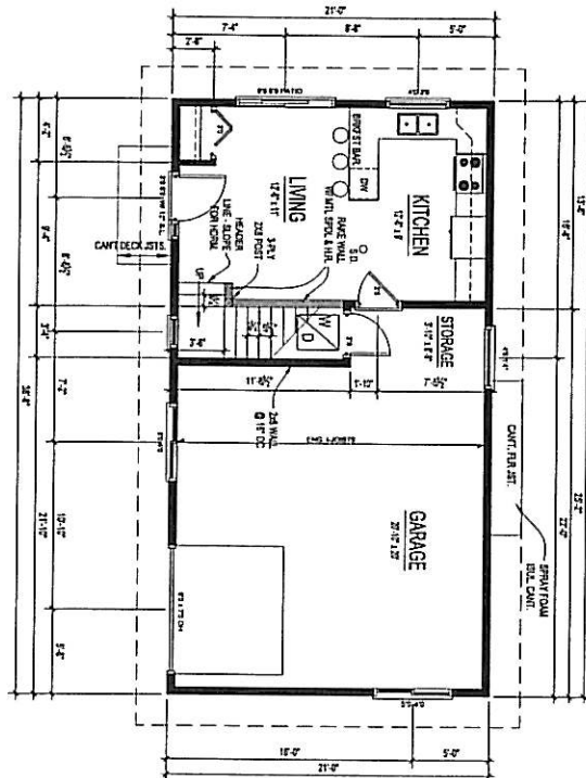
MAIN FLOOR PLAN 3/12/17 SCALE: 1/8" = 1'-0"
